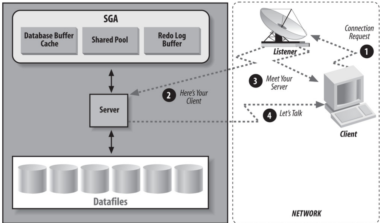
Figure 3-3. Connecting with the Oracle Net Listener
