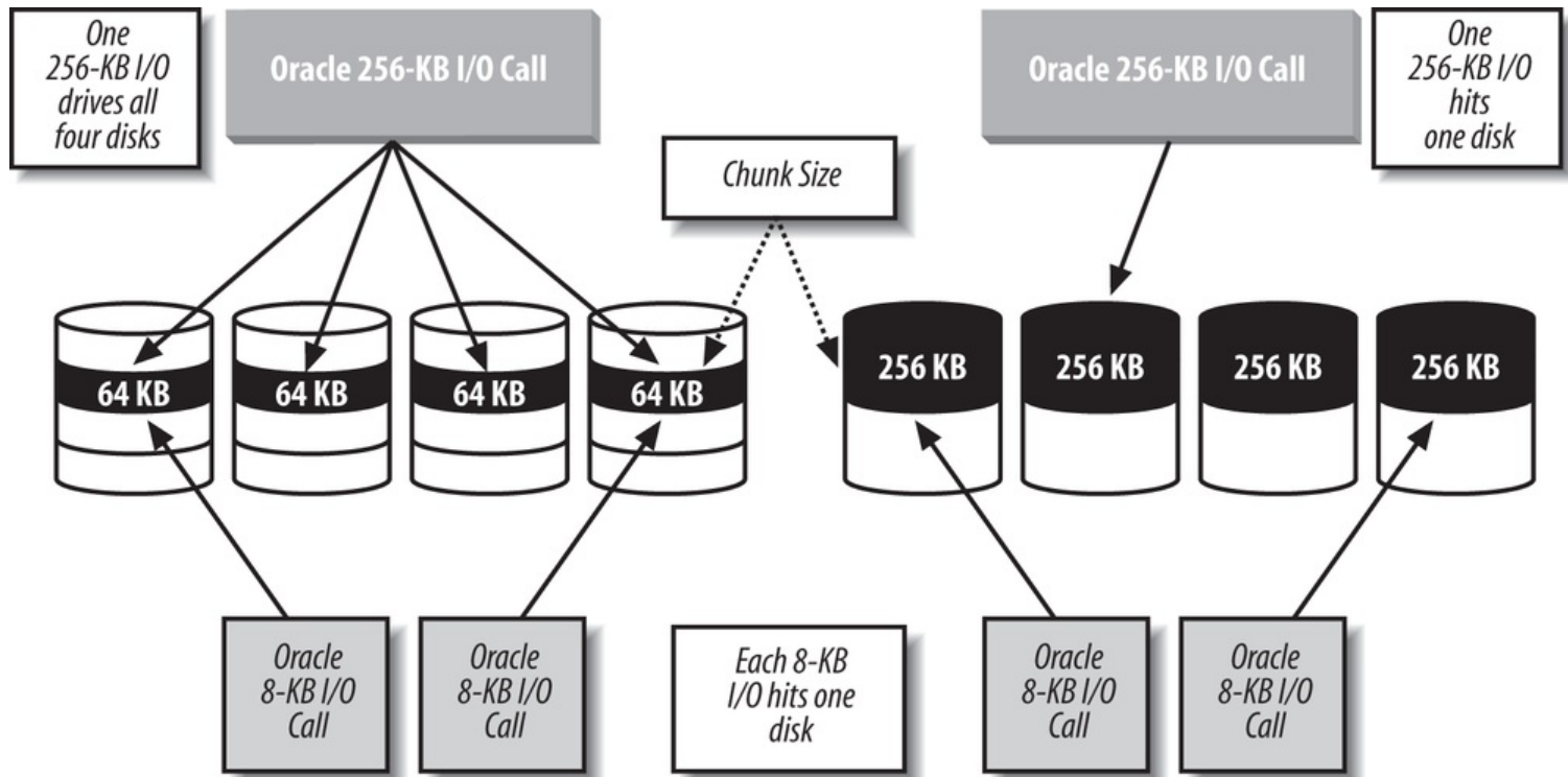
Figure 7-4. Intra-operation and inter-operation parallelism
