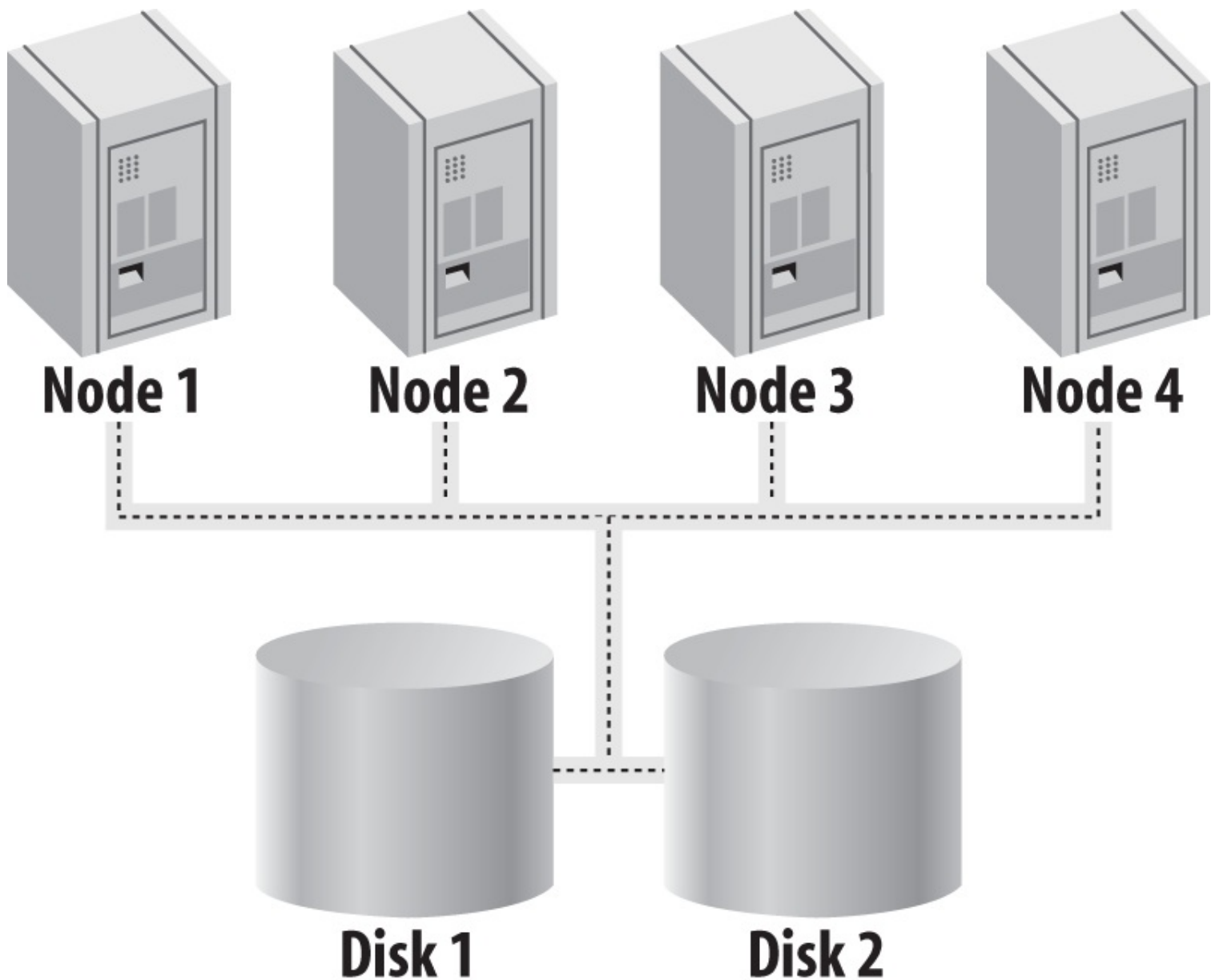
Figure 9-6. RAC architecture
