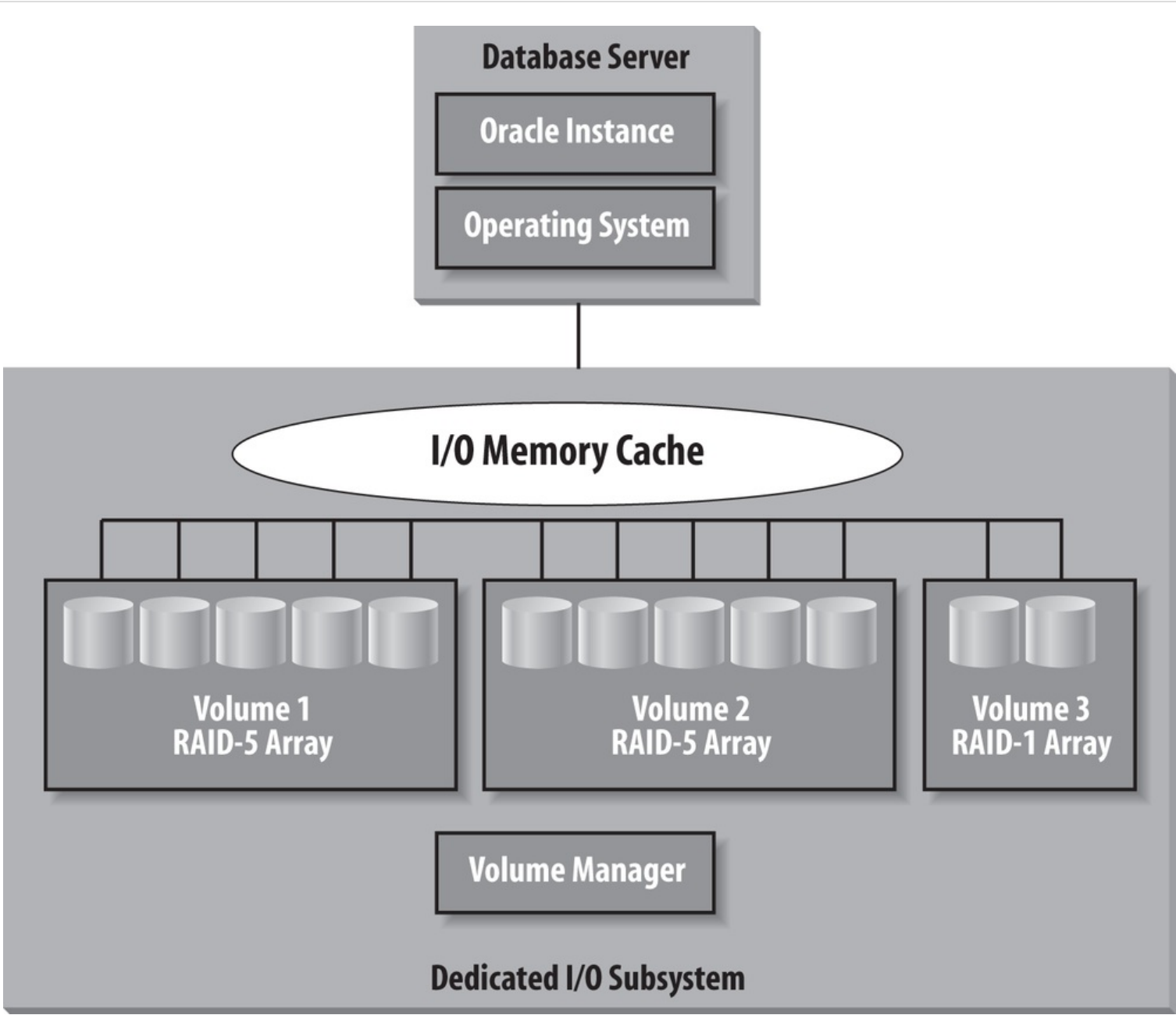
Figure 7-2. Dedicated I/O subsystems
