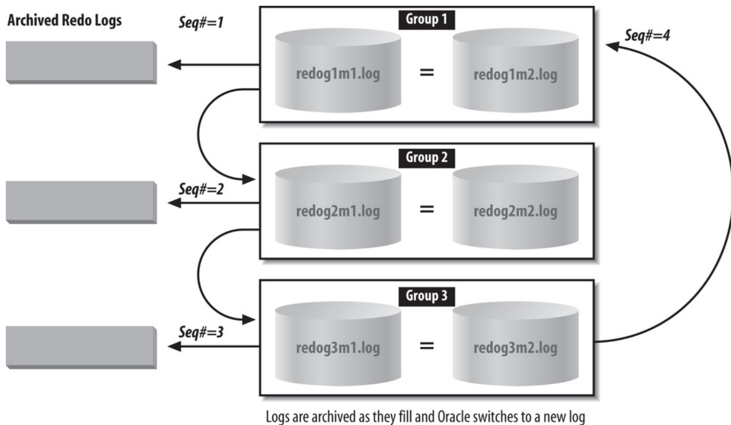
Figure 2-7. Cycling redo logs with archiving
